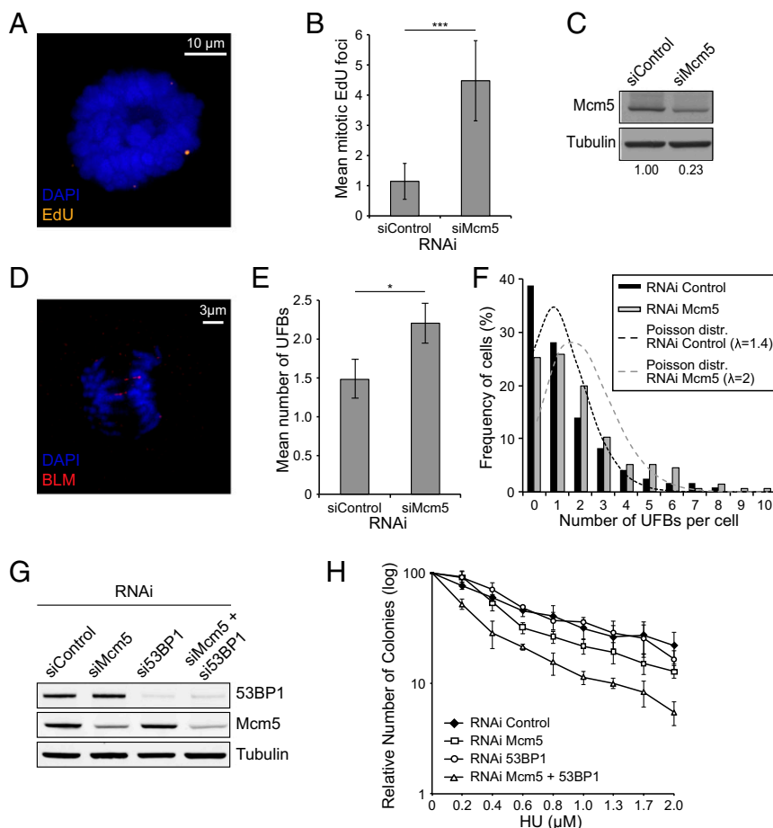
Fig. 4. MCM5 RNAi effects on mitosis. (A) Representative image of early-mitotic HeLa cell with foci of EdU incorporation. (B) Quantification of foci of EdU incorporation during prophase and prometaphase HeLa cells after MCM5 RNAi ( n = 100 , three replicates, error bars are SEM). t test, P = 3.43 \times 10^{-8} . (C) Immunoblot to show depletion of MCM5 after MCM5 RNAi. Quantification of band intensity is indicated below the blot. (D) Representative image of UFBs stained with BLM in an anaphase HeLa cell. (E) Frequency of UFBs after 48-h treatment with MCM5 RNAi ( n = 75 , three replicates, error bars are SEM). t test, P = 0.0473 . (F) Frequency distribution of UFBs ( n = 100 cells, four replicates). \chi^2 tests for Poissons, P > 0.85 . A significant difference was observed. Wilcoxon rank sum test, P = 5.095 \times 10^{-3} . (G) Immunoblot showing the knockdown of MCM5 and 53BP1 by RNAi in HeLa cells. (H) Clonogenic assay after treatment, as seen in G, with increasing HU (three replicates, error bars are SEM).
