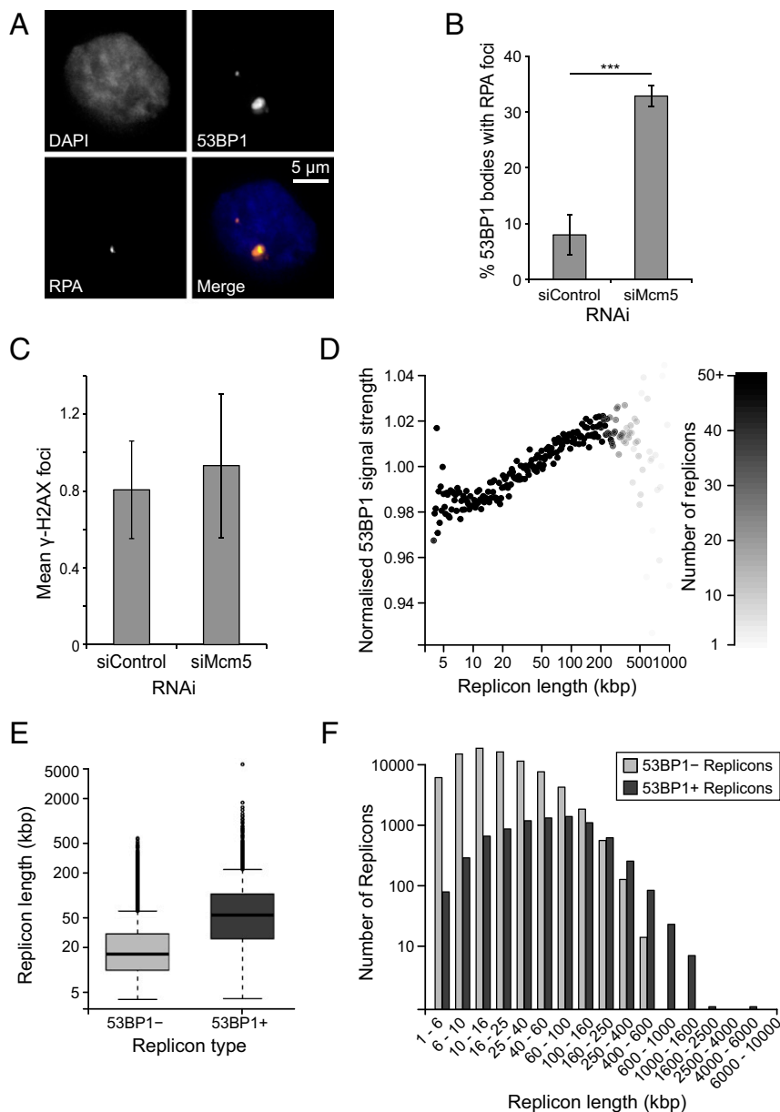
Fig. 3. The 53BP1 is enriched at genomic loci that correspond to large replicons. (A) Representative image of the colocalization between G1-specific 53BP1 nuclear bodies and RPA foci. (B) Percentage of total cellular 53BP1 nuclear bodies that colocalize with RPA after treatment with control or MCM5 RNAi ( n = 100 , three replicates, error bars are SEM). t test, P = 3.01 \times 10^{-3} . (C) Mean frequency of G1-specific \gamma -H2AX foci in HeLa cells after MCM5 RNAi ( n = 150 , three replicates, error bars are SEM). t test, P = 0.585 . (D) Plot of the average 53BP1/IgG signal ratio per kilobase against replicon size. A strong and significant correlation is observed (Spearman \rho = 0.91 , P < 10^{-15} ). (E) Distribution of the size of 53BP1+ and 53BP1- replicons. t test, P < 10^{-15} . (F) Frequency distribution of 53BP1+ and 53BP1- replicons across different replicon sizes. \chi^2 test, P < 10^{-15} .
