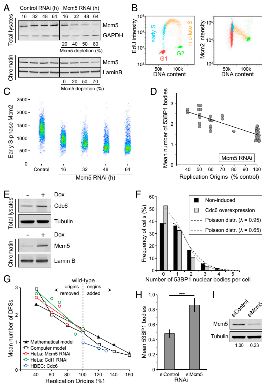
Fig. 2. Origin number and the frequency of 53BP1 nuclear bodies. (A) Immunoblot of total and chromatin-bound MCM5 in HeLa cells after MCM5 RNAi. (B) Three-dimensional FACS of HeLa cells labeled with EdU ( Left ) and MCM2 ( Right ). Red, G1 phase: EdU negative and G1 DNA content. Blue, early S phase: incorporation of EdU without significant increase in total DNA content. Orange, late S phase: EdU positive cells with >G1 DNA content. Green, G2 phase: EdU negative and G2 DNA content. (C) FACS of chromatin-associated MCM2 signal in early S phase HeLa cells with indicated periods of MCM5 RNAi. (D) Frequency of G1-specific 53BP1 nuclear bodies (y-axis values) after MCM5 knockdown versus relative number of replication origins quantified by 3D FACS of DNA-bound MCM2 (x-axis values). Each point represents the mean of 100 cells. (E and F) CDC6-inducible HEBC cells. Immunoblot of CDC6 and tubulin in whole-cell lysates (E, Top ) and MCM5 and Lamin B1 in chromatin samples (E, Bottom ). Frequency distribution of 53BP1 nuclear bodies in HEBC cells (F) ( n = 100 , three replicates). \chi^2 tests for fitted Poissons, P > 0.87 . The two conditions are significantly different (Wilcoxon rank sum test, P = 2.843 \times 10^{-6} ). (G) Compilation of the predicted number of DFSs using the mathematical model and the computer simulation (from Fig. 1B) and the mean number of 53BP1 nuclear bodies in vivo (from D and F and Fig. S2E). (H) Frequency of G1-specific 53BP1 nuclear bodies in control and MCM5 RNAi-treated IMR-90 cells ( n = 150 , three replicates, error bars are SEM). t test, P = 1.79 \times 10^{-4} . (I) Immunoblot to show the depletion of MCM5 after RNAi. Quantification of band intensity is indicated below the blot.
