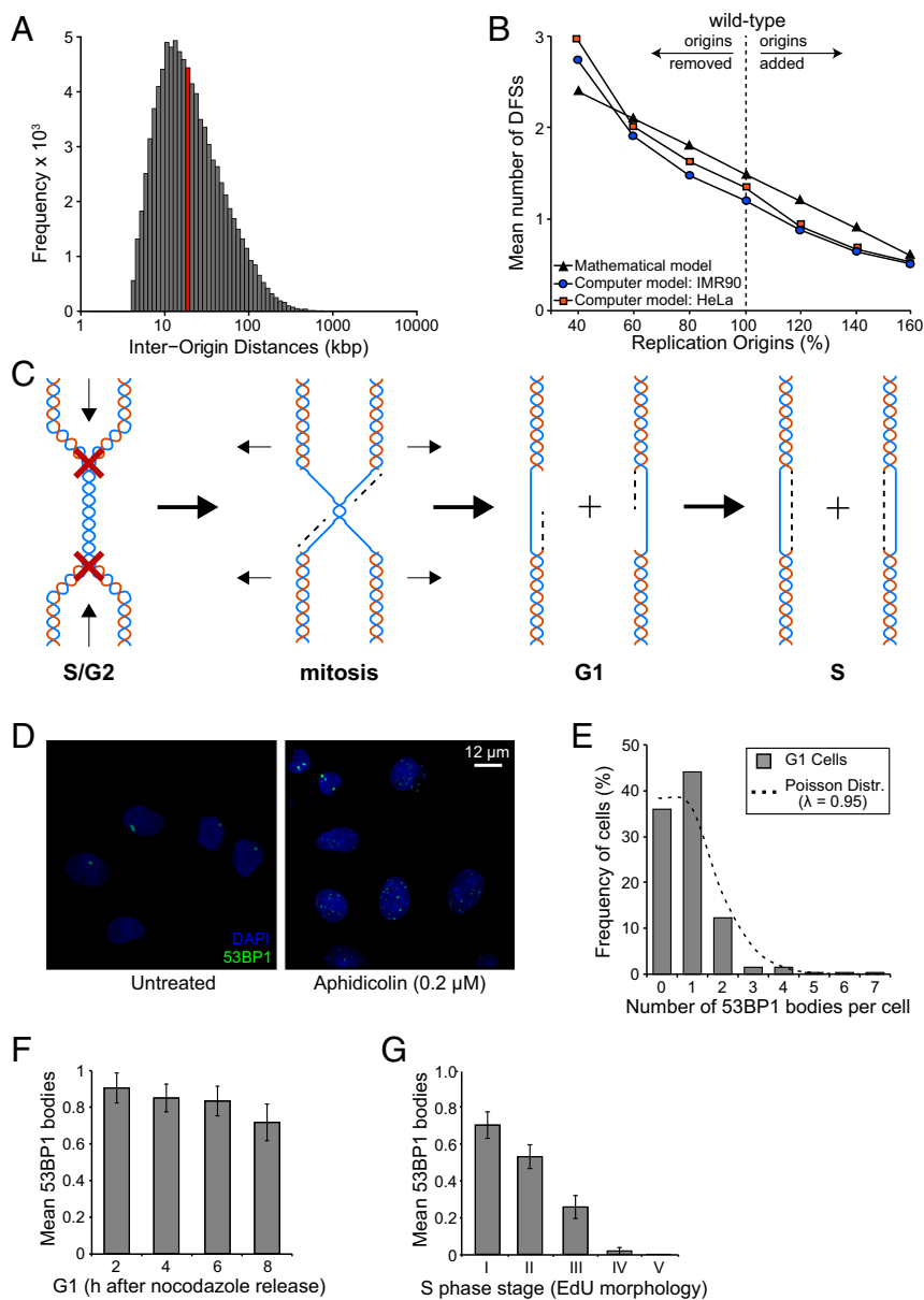
Fig. 1. Potential mechanism for resolution of DFSS. (A) Distribution of replicon sizes in HeLa cells, based on data from ref. 13. The red bar represents the average replicon size of \sim 31 kb. (B) Mean number of DFSS predicted using a mathematical model (4), and a computational model that uses origin data from HeLa and IMR-90 (13) when origins are added or depleted randomly. (C) Model for segregation of unreplicated DNA to daughter cells for resolution in the next cell cycle. (D) The 53BP1 nuclear bodies in untreated and aphidicolin-treated cells. (E) Frequency of G1-specific 53BP1 nuclear bodies ( n = 100 , three replicates). \chi^2 test for a fitted Poisson, P = 0.771 . (F) Frequency of G1-specific 53BP1 nuclear bodies at the times indicated after nocodazole treatment and mitotic shake-off ( n = 150 , three replicates, error bars are SEM). \chi^2 test, P = 0.924 . (G) Frequency of 53BP1 nuclear bodies at different stages of the replication timing program, as defined by O'Keefe et al. (32) ( n = 150 , three replicates, error bars are SEM). \chi^2 test, P = 4.998 \times 10^{-4} .
