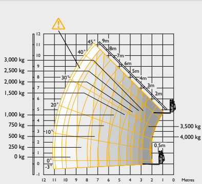
540-180 HiViz Stabilisers retracted Sway
