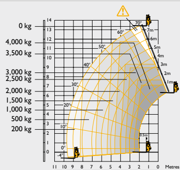
540-140 HiViz Stabilisers retracted Sway
