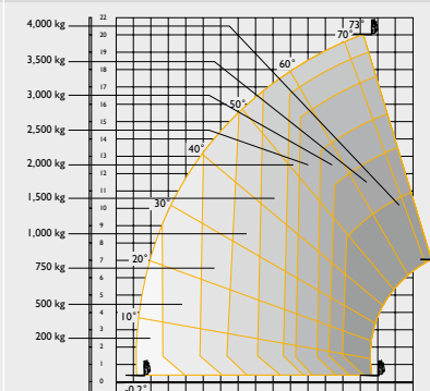
540-200 Stabilisers extended Sway
